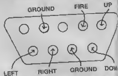
Spectrum Plus Two joystick socket wiring (view of socket 1 or 2)
